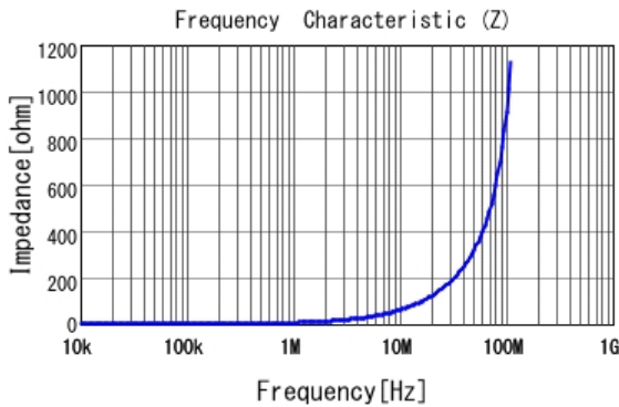
■ LQH2HPN1R0NJR |Z|
