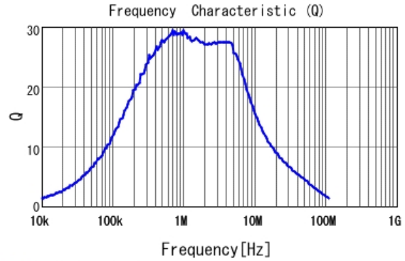
■ LQH2HPN1R0NJR Q
