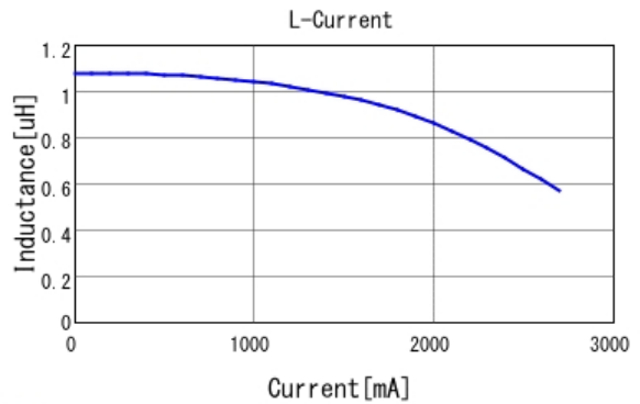
■ LQH2HPN1R0NJR L-Current 20degC
