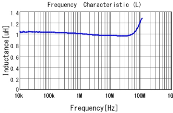
■ LQH2HPN1R0NJR L
