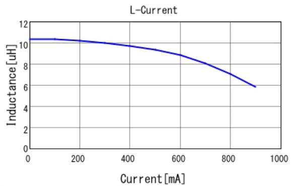
■ LQH2HPN100MJR L-Current 20degC
