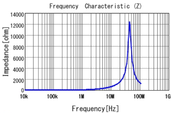
■ LQH2HPN100MJR |Z|
