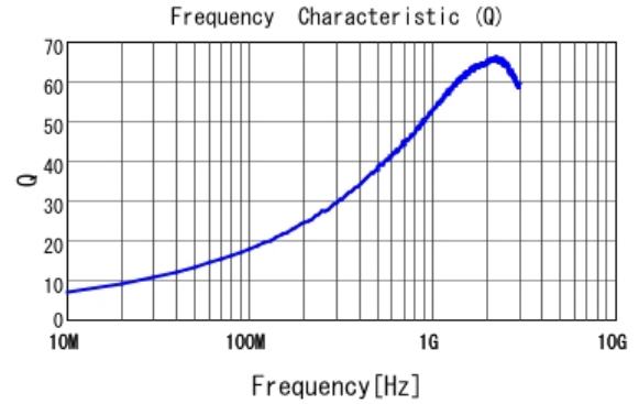
■ LQG15WZ6N8J02 Q
