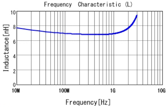
■ LQG15WZ6N8J02 L
