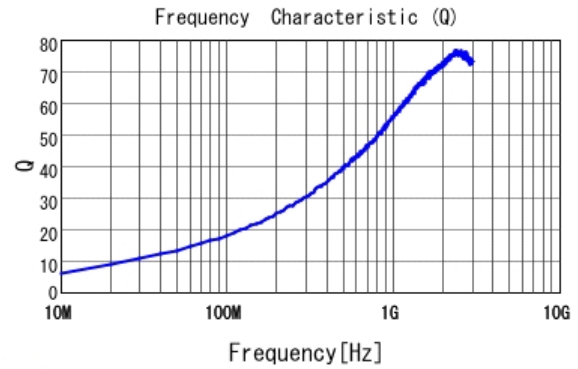
■ LQG15WZ5N6C02 Q
