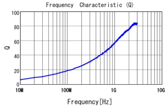
■ LQG15WZ3N9S02 Q
