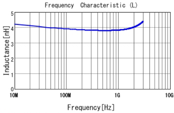
■ LQG15WZ3N9S02 L
