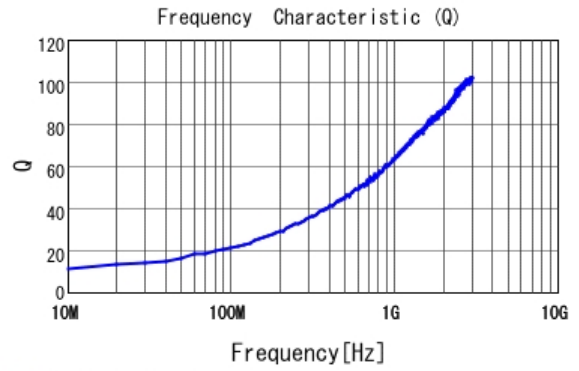
■ LQG15WZ2N7S02 Q
