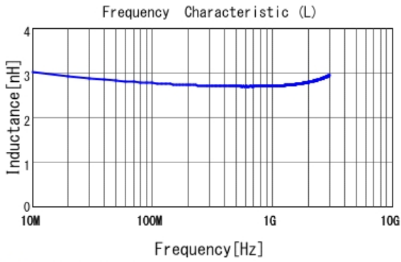
■ LQG15WZ2N7S02 L
