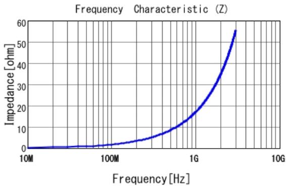
■ LQG15WZ2N7C02 |Z|
