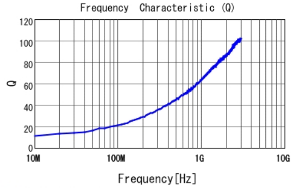
■ LQG15WZ2N7C02 Q
