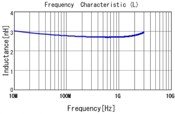
■ LQG15WZ2N7C02 L
