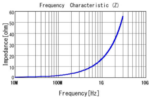
■ LQG15WZ2N7B02 |Z|
