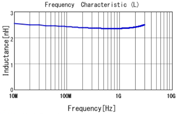
■ LQG15WZ2N4B02 L
