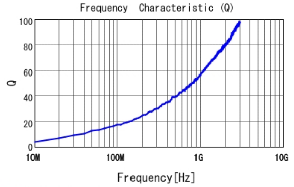
■ LQG15WZ2N4B02 Q
