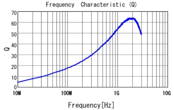
■ LQG15WH9N1J02 Q
