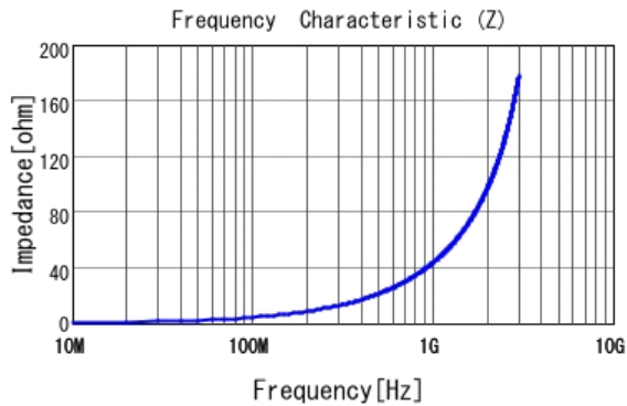
■ LQG15WH6N8J02 |Z|
