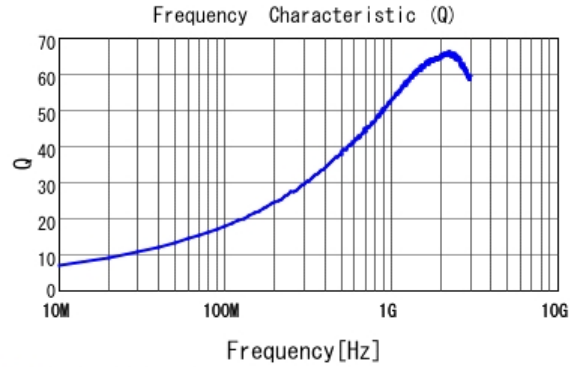
■ LQG15WH6N8J02 Q
