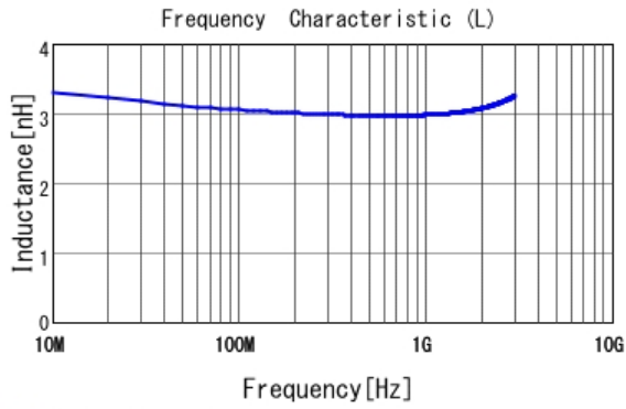
■ LQG15WH3N0B02 L
