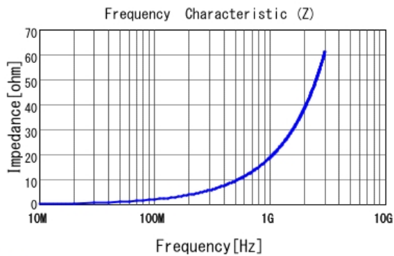
■ LQG15WH3N0B02 |Z|
