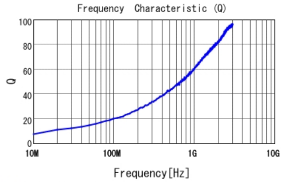
■ LQG15WH3N0B02 Q
