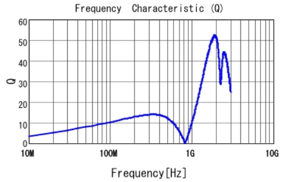
■ LQG15HSR15G02 Q
