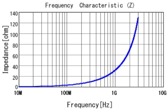
■ LQG15HS5N1B02 |Z|
