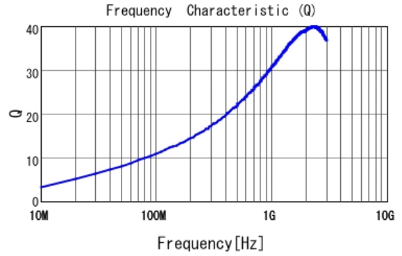
■ LQG15HS5N1B02 Q
