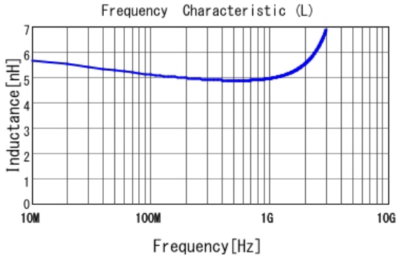
■ LQG15HS5N1B02 L
