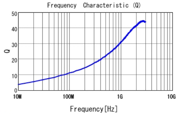
■ LQG15HS3N9C02 Q
