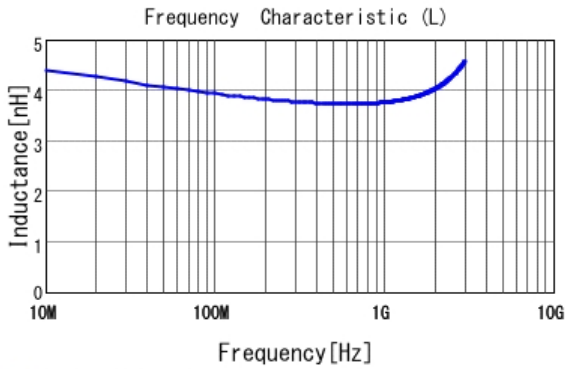
■ LQG15HS3N9C02 L
