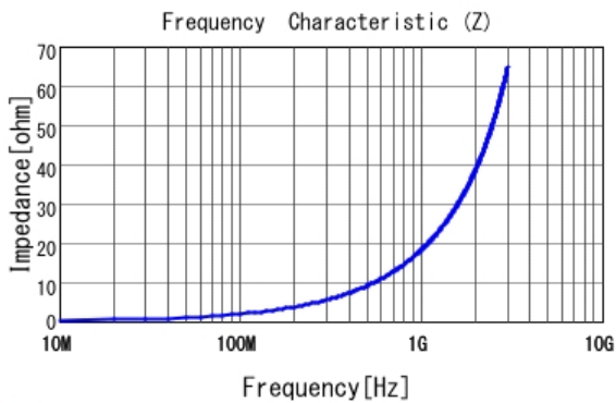
■ LQG15HS3N0B02 |Z|
