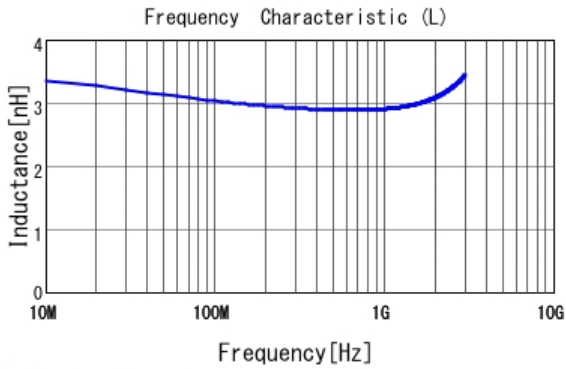
■ LQG15HS3N0B02 L
