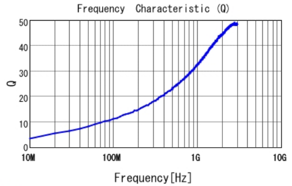
■ LQG15HS3N0B02 Q
