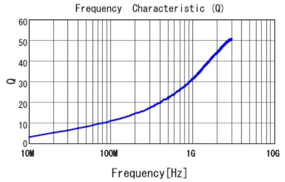
■ LQG15HS2N4C02 Q
