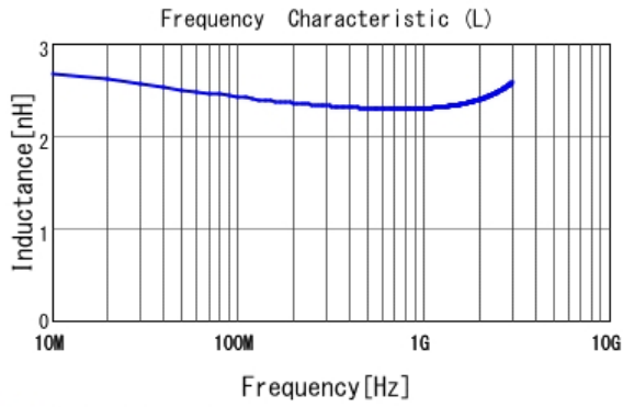
■ LQG15HS2N4C02 L
