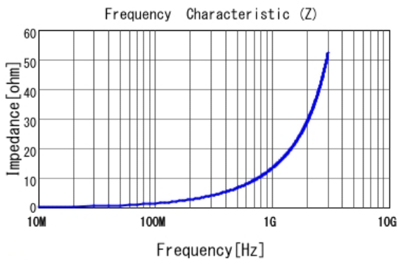
■ LQG15HS2N2C02 |Z|
