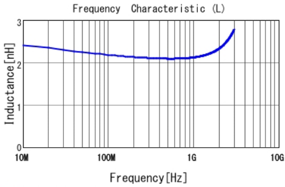
■ LQG15HS2N2C02 L
