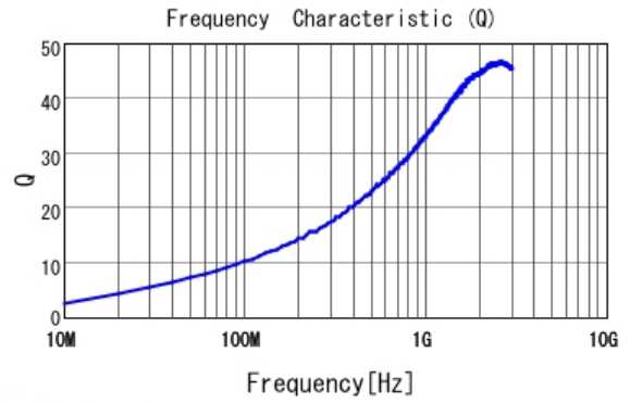
■ LQG15HS2N2C02 Q
