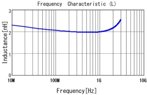
■ LQG15HS2N0B02 L
