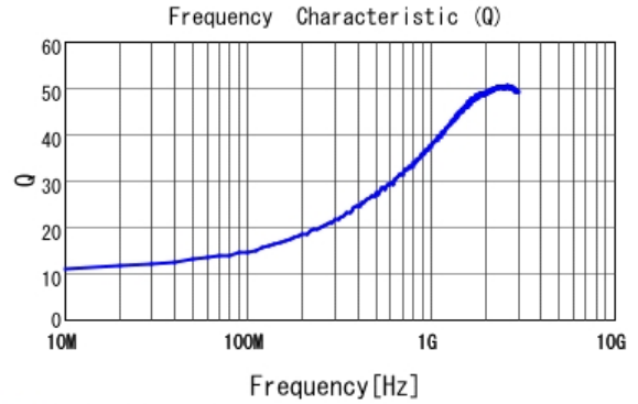
■ LQG15HS2N0B02 Q
