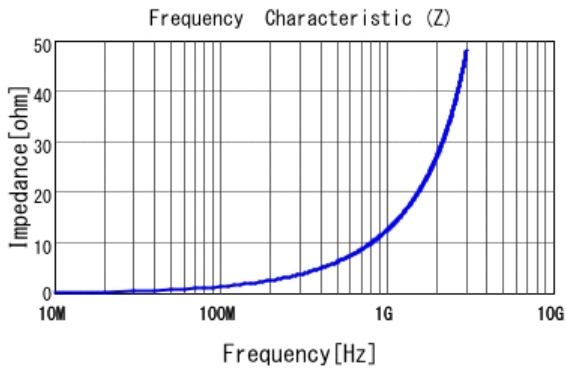
■ LQG15HS2N0B02 |Z|
