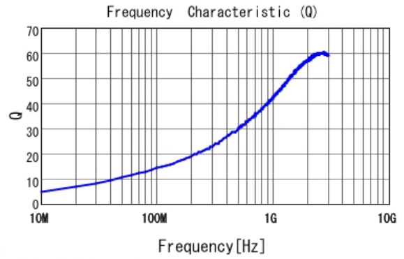
■ LQG15HN2N4C02 Q
