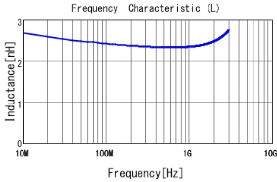
■ LQG15HN2N4C02 L
