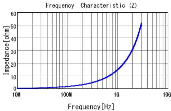
■ LQG15HN2N4C02 |Z|
