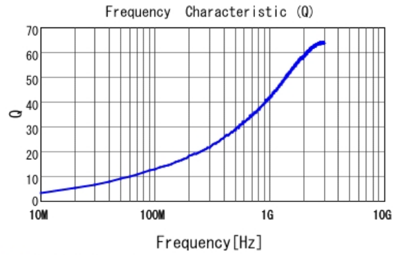
■ LQG15HN2N2C02 Q
