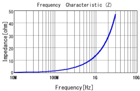
■ LQG15HN2N2C02 |Z|
