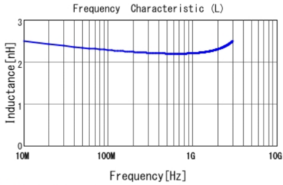
■ LQG15HN2N2C02 L
