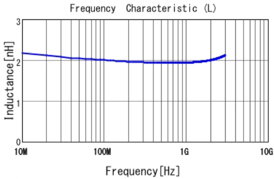
■ LQG15HN2N0B02 L
