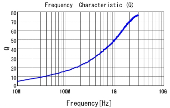
■ LQG15HN2N0B02 Q
