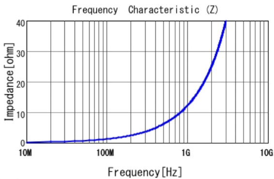
■ LQG15HN2N0B02 |Z|
