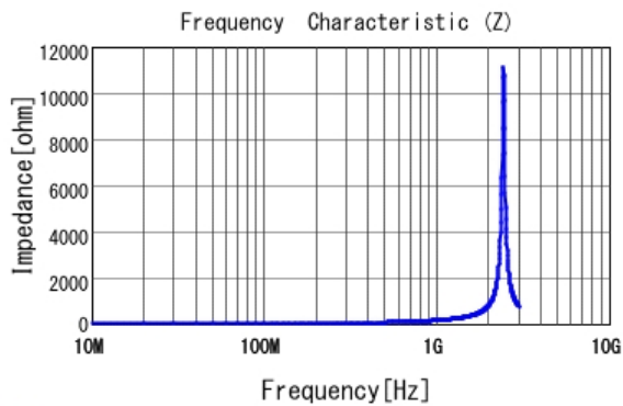
■ LQG15HN22NG02 |Z|
