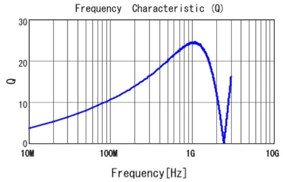
■ LQG15HN22NG02 Q
