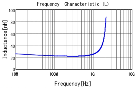
■ LQG15HN22NG02 L
