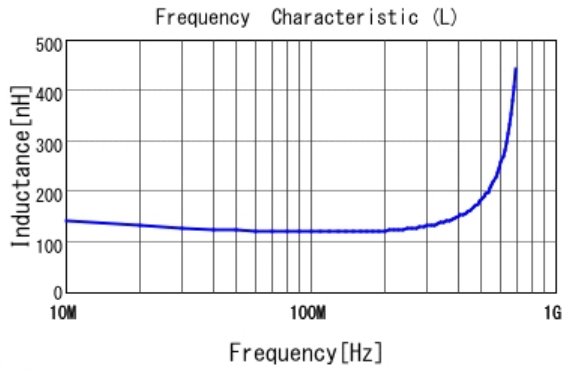
■ LQG15HHR12G02 L
