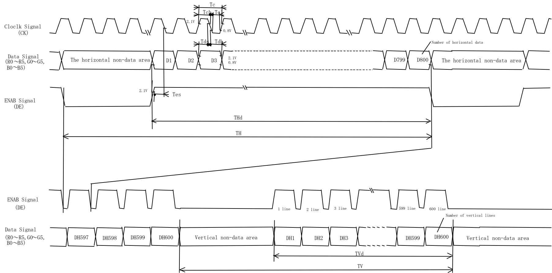
Fig2 Input signal timing
