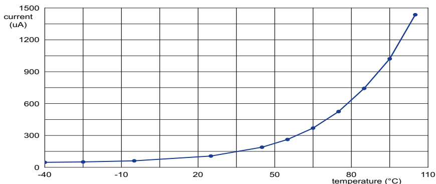
Fig 8. Deep-sleep mode: Typical supply current I_{DD} versus temperature for different supply voltages VBAT_DCDC
