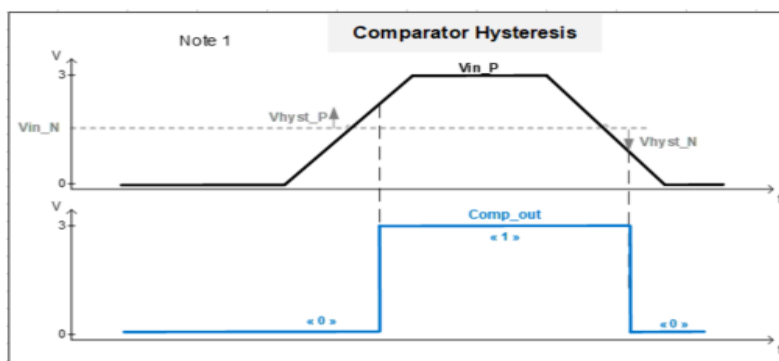
Fig 22. Comparator Hysteresis
