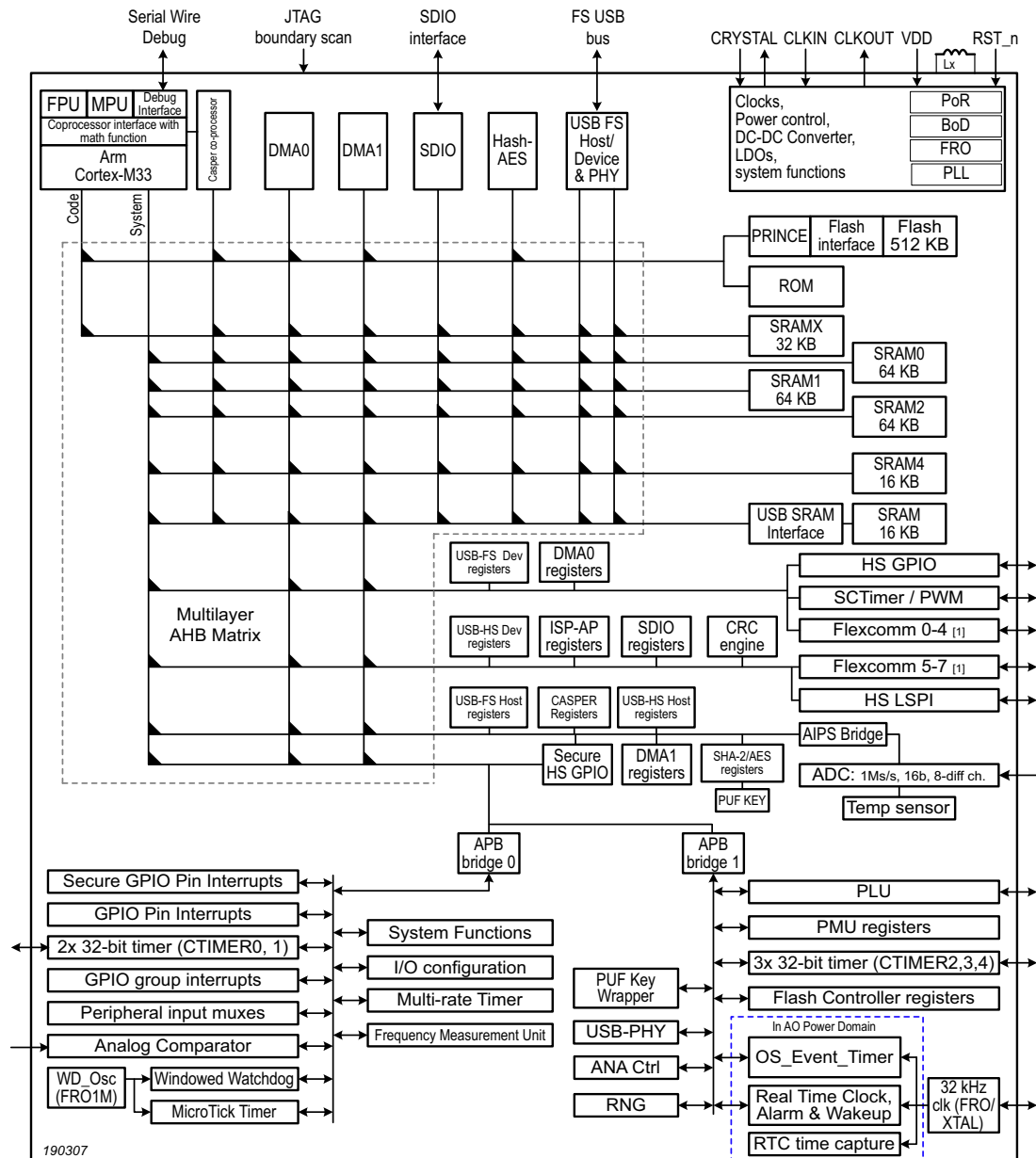
Fig 3. LPC55S2x/LPC552x Block Diagram
