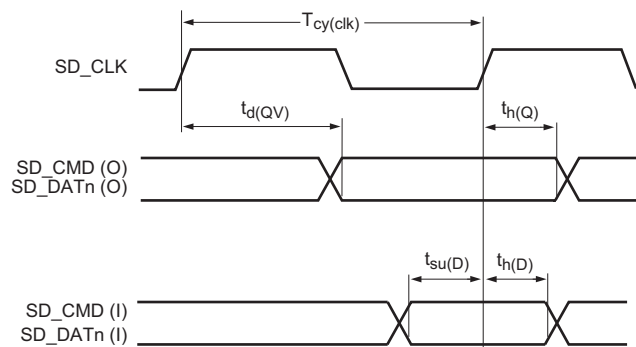
Fig 20. SD/MMC and SDIO timing
