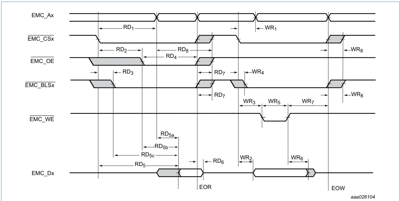
Fig 25. External static memory read/write access (PB = 1)
