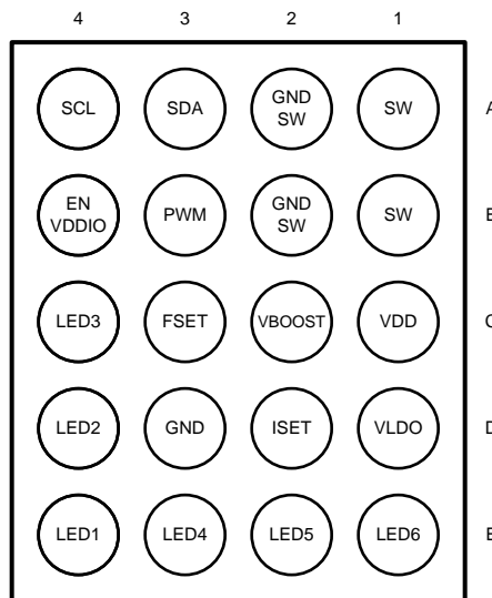
20-Pin DSBGA Package Bottom View
