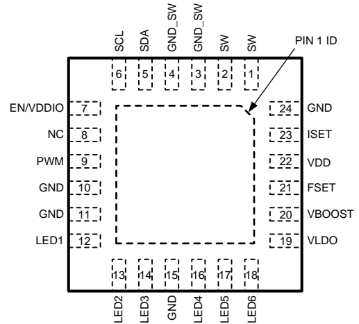
24-Pin WQFN Package Top View
