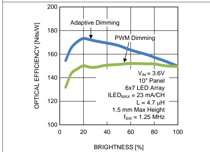
Figure 24. Optical Efficiency
