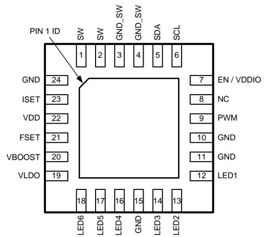
24-Pin WQFN Package Bottom View
