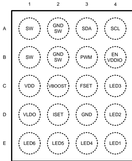
20-Pin DSBGA Package Top View
