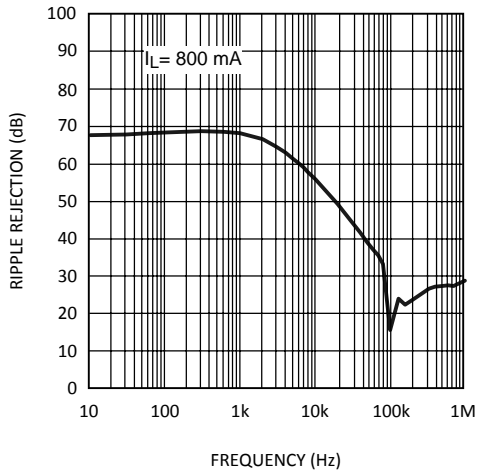
Figure 9. Ripple Rejection
