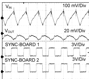
Figure 53. Output voltage ripple of two modules with synchronization clocks 180 degrees out of phase
