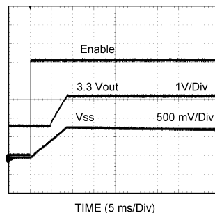
Figure 54. Pre-Biased Startup
