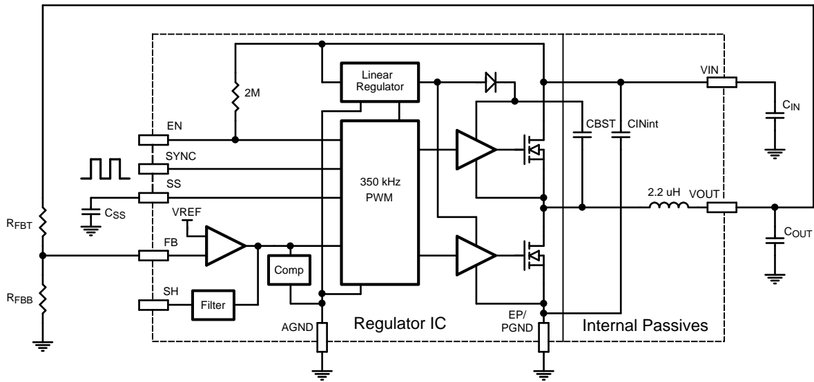
Figure 47. Block Diagram
