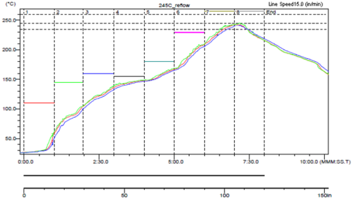
Figure 58. Sample Reflow Profile
