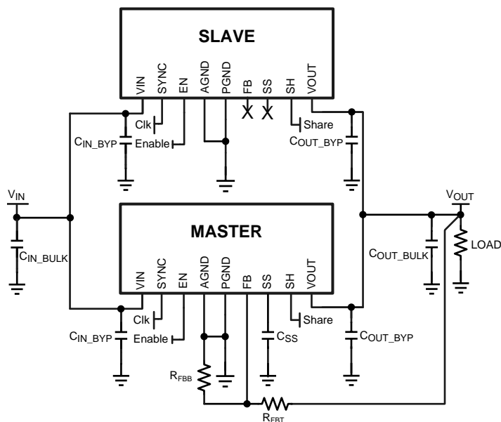
Figure 51. Current Sharing Example Schematic
