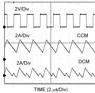
Figure 55. CCM and DCM Operating Modes V_{IN} = 12V, V_O = 3.3V, I_O = 3A/0.3A
