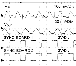
Figure 53. Output voltage ripple of two modules with synchronization clocks 180 degrees out of phase
