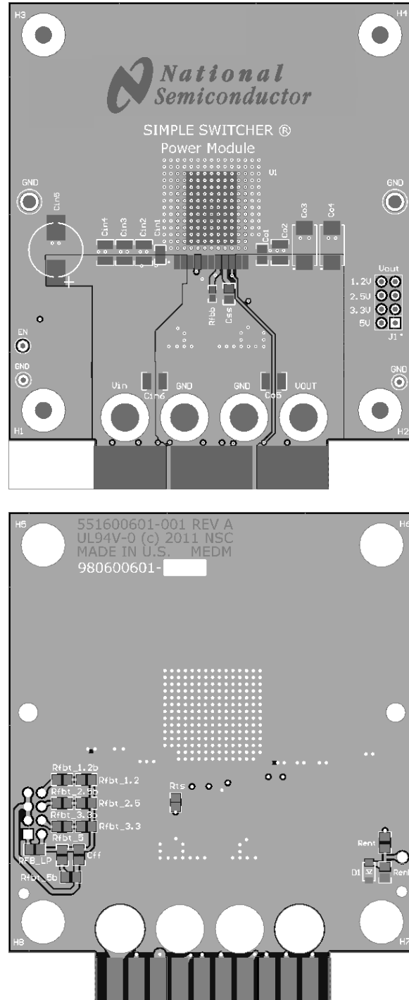
Figure 57. Layout example
