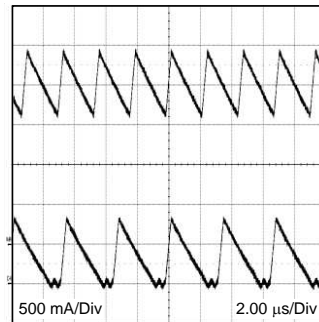
Figure 33. CCM and DCM Operating Modes V_{IN} = 24V , V_O = 3.3V , I_O = 2A/0.32A 2 \mu\text{sec/div}
