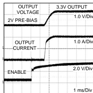
Figure 35. Pre-Biased Startup
