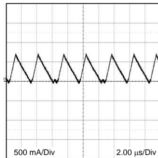
Figure 34. Transition Mode Operation V_{IN} = 24V , V_O = 3.3V , I_O = 0.35A 2 \mu\text{sec/div}
