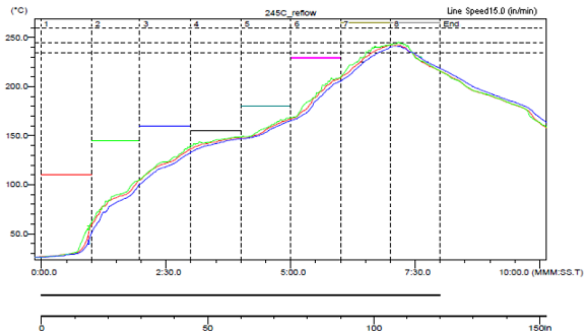
Figure 37. Sample Reflow Profile
