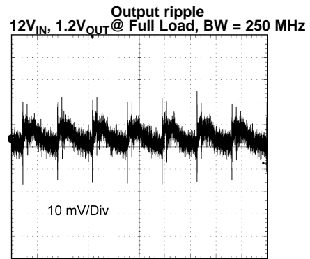
TIME (2 \mu s /Div) Figure 43.
