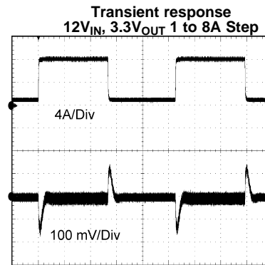
TIME (500 \mu s /Div) Figure 45.
