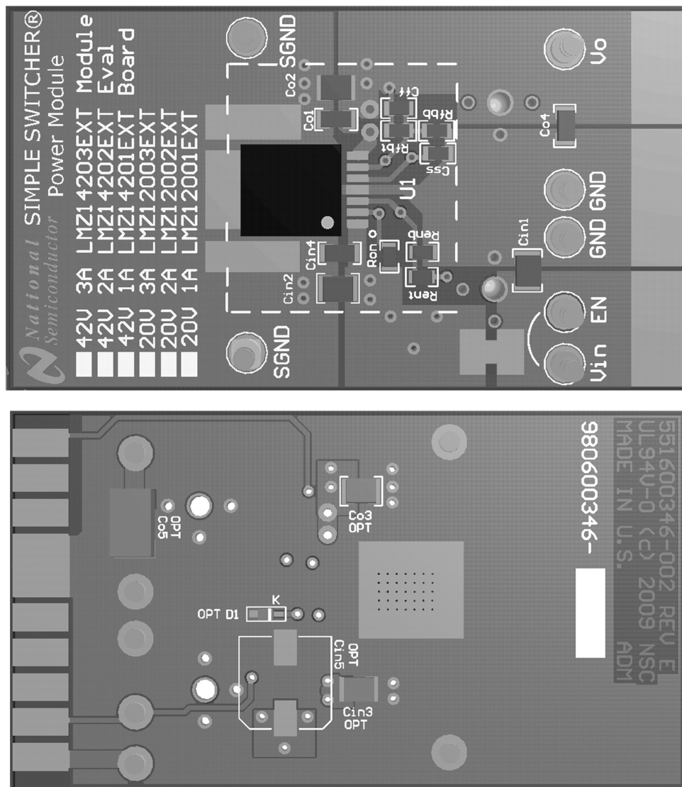
Figure 27. PCB Layout Example
