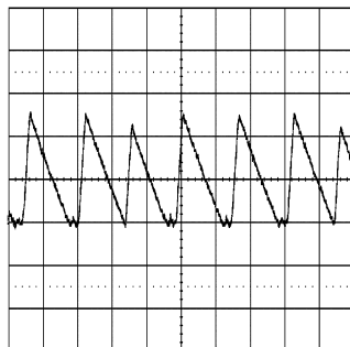
Figure 25. Transition Mode Operation V_{IN} = 12V, V_O = 3.3V, I_O = 0.5 A \ 2 \ \mu\text{sec/div}
