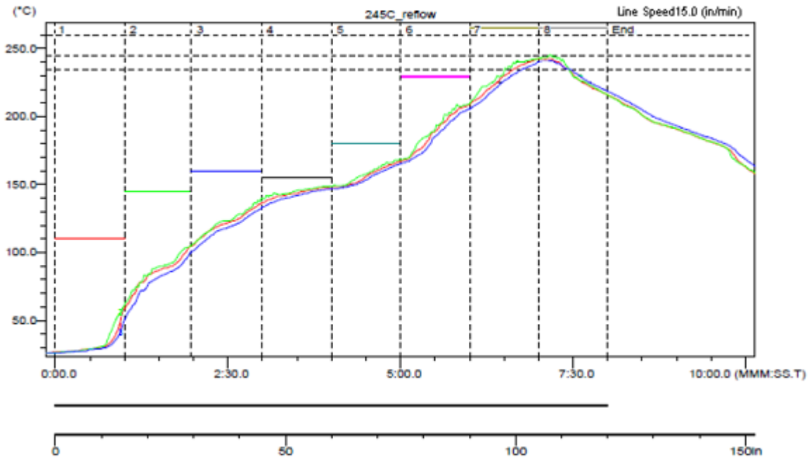
Figure 28. Sample Reflow Profile
