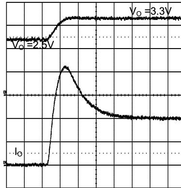
Figure 26. Pre-Biased Startup
