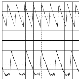
Figure 24. CCM and DCM Operating Modes V_{IN} = 12V, V_O = 3.3V, I_O = 3A/0.4A \ 2 \ \mu\text{sec/div}
