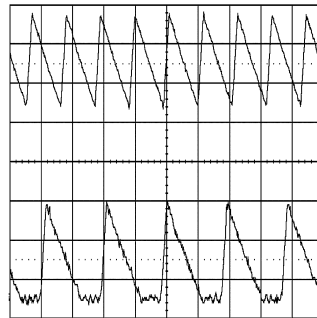
Figure 40. CCM and DCM Operating Modes V_{IN} = 12\text{V}, V_O = 3.3\text{V}, I_O = 1\text{A}/0.25\text{A}
