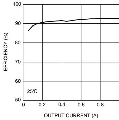
Figure 2. Efficiency V_{IN} = 12V V_{OUT} = 5.0V
