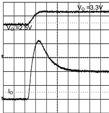
Figure 42. Pre-Biased Startup
