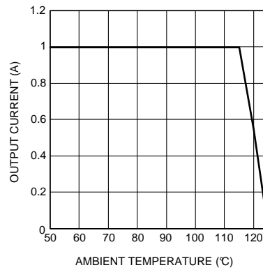
Figure 3. Thermal Derating Curve V_{IN} = 12V V_{OUT} = 5.0V
