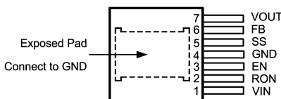
Figure 5. 7-Pin PFM (Top View) See NDW0007A Package
