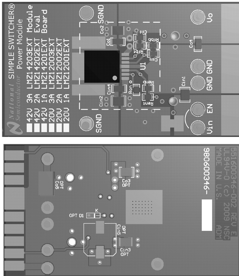
Figure 43. Top And Bottom View Of Evaluation PCB
