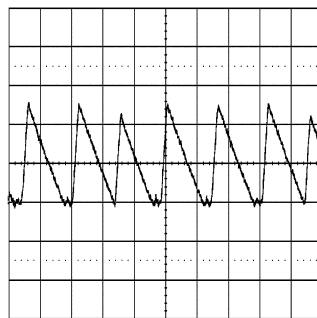
Figure 41. Transition Mode Operation V_{IN} = 12\text{V}, V_O = 3.3\text{V}, I_O = 0.29\text{A}
