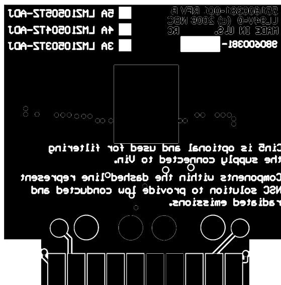
Figure 29. Bottom Copper
