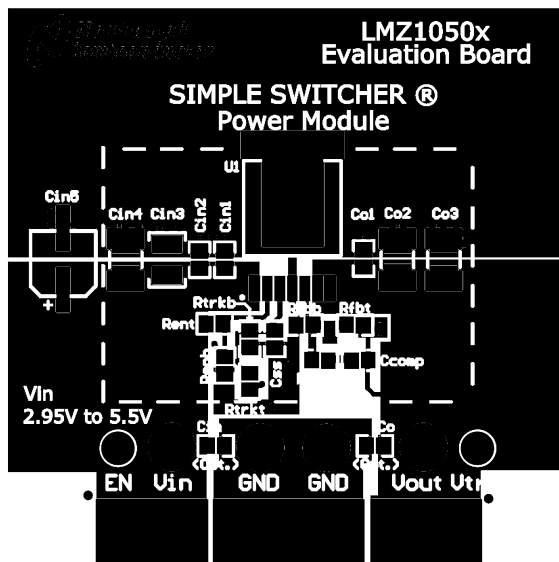
Figure 26. Top Copper
