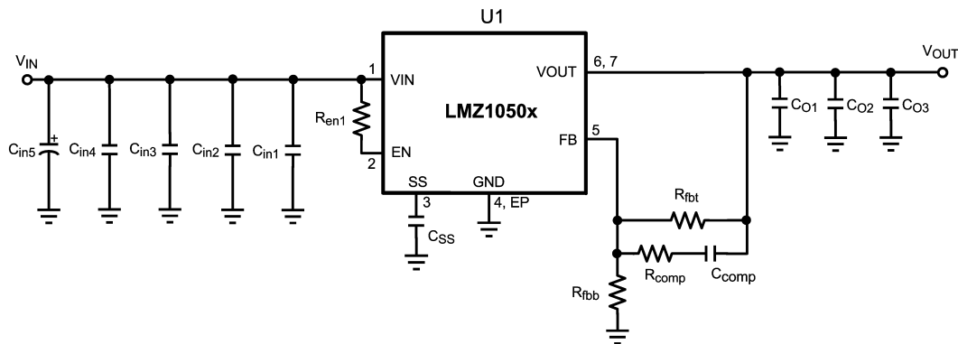
Figure 1. Component Schematic for Evaluation Board
