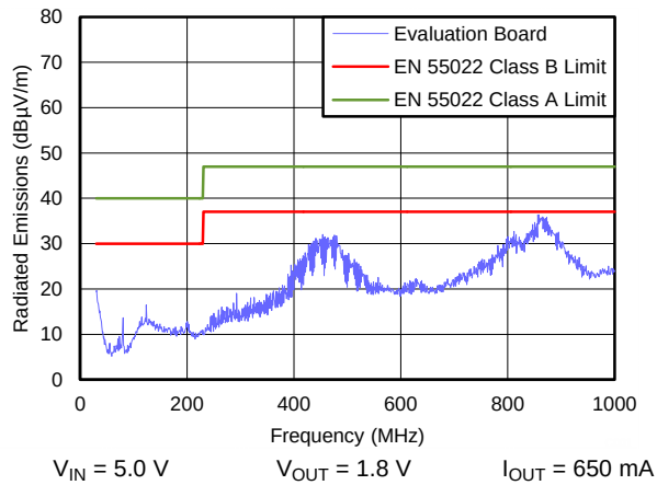
Figure 7. Radiated EMI (CISPR22) Default Evaluation Board BOM
