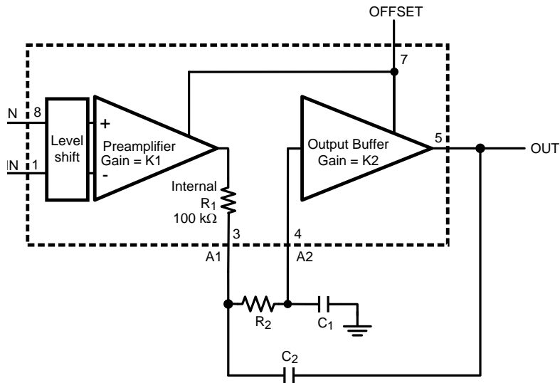
Figure 38. Second Order Low Pass Filter
