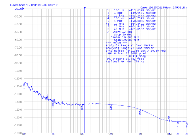
Figure 1. Closed Loop Phase Noise of LVPECL Differential Output at 156.25 MHz with PLL bandwidth at 400 kHz, Integer-N PLL, 5 GHz VCO Frequency, Output Divider = 32
