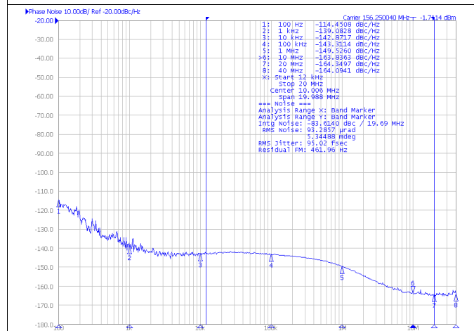
Figure 3. Closed Loop Phase Noise of HCMSEL Differential Output at 156.25 MHz with PLL bandwidth at 400 kHz, Integer-N PLL, 5 GHz VCO Frequency, Output Divider = 32
