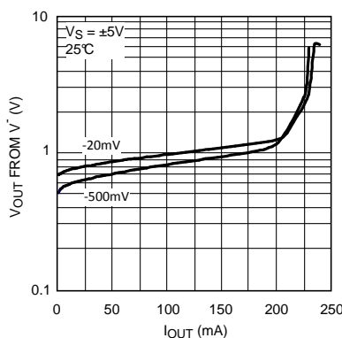
Figure 54. V_{OUT} vs. I_{SINK} (for Various Overdrive)
