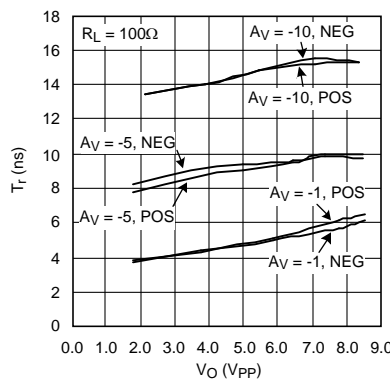
Figure 52. Output 20%-80% Transition vs. Output Voltage Swing (Inverting Gain)
