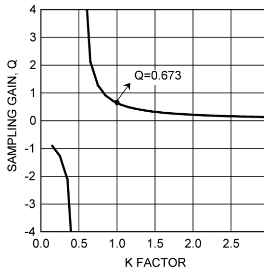
Figure 38. Sampling Gain Q vs K Factor
