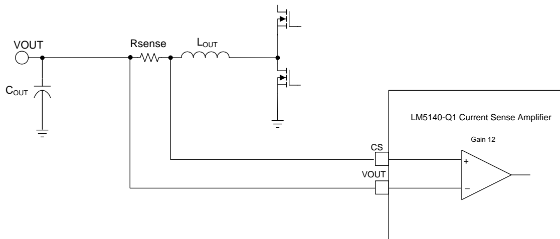
Figure 28. Current Sense
