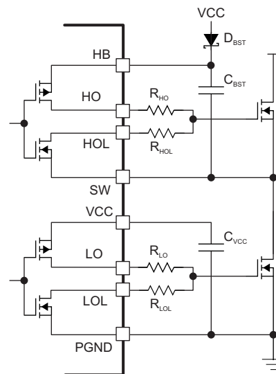
Figure 31. Drivers
