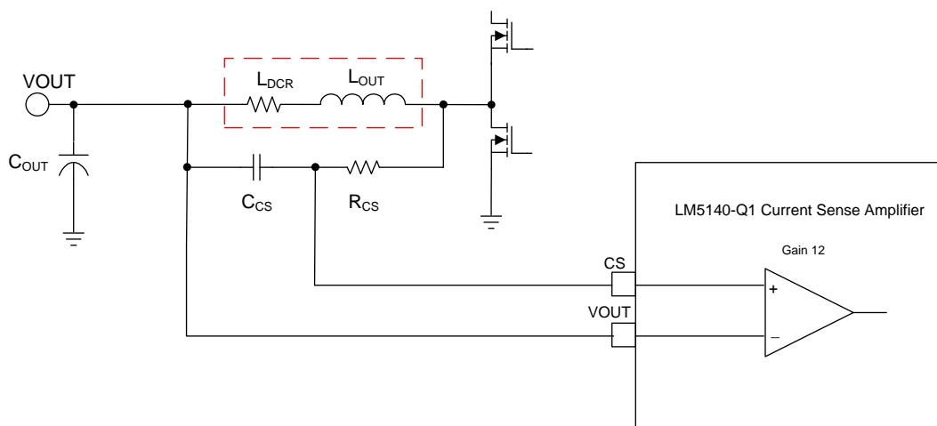
Figure 29. DCR Current Sensing
