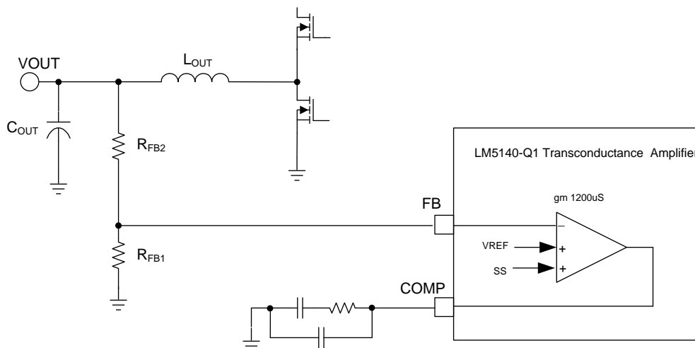
Figure 27. Voltage Feedback
