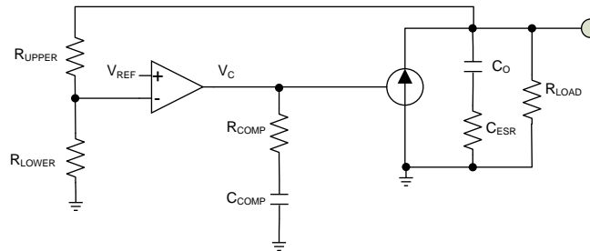
Figure 39. Transconductance Amplifier
