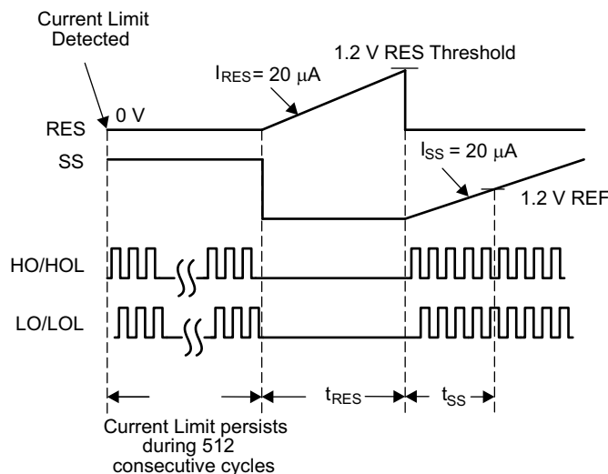
Figure 30. Hiccup Mode
