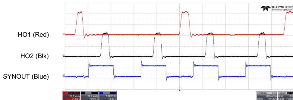
Figure 22. HO1, HO2, and SYNOUT VIN 36 V
