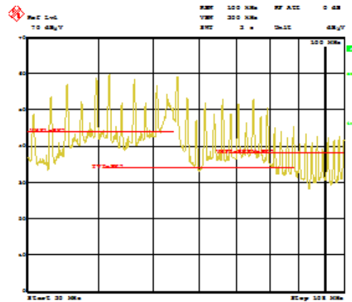
Figure 35. EMI Measurements CISPR 25, No Slew Rate Control
