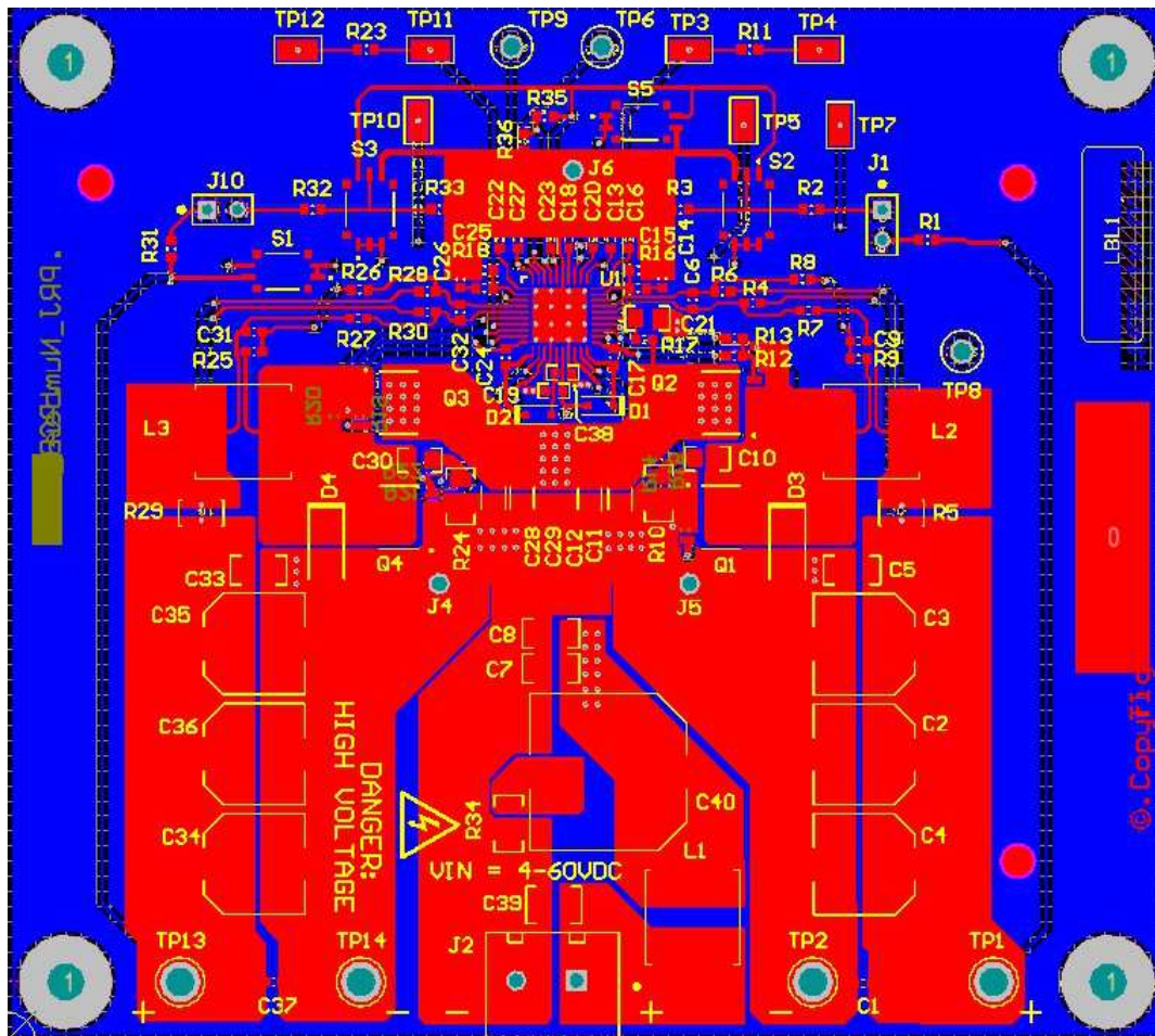
Figure 45. Top/Bottom PWM Layers
