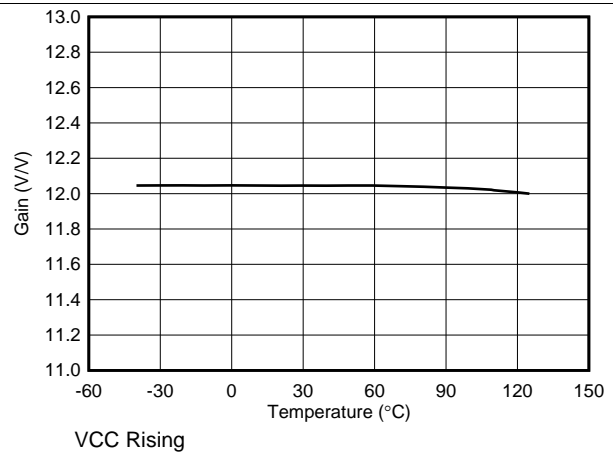
Figure 13. Current Sense Amplifier Gain vs Temperature
