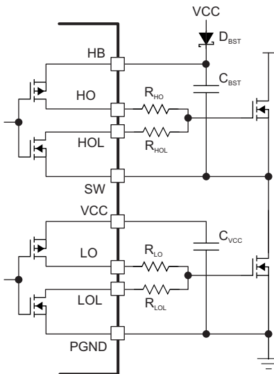
Figure 34. Drivers with Slew Rate Control
