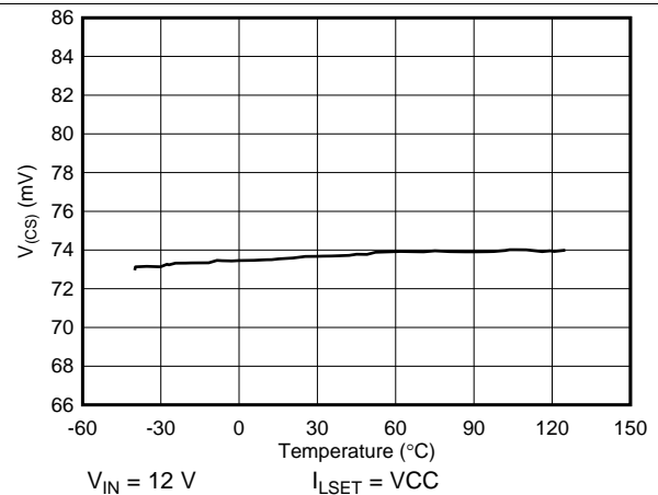
Figure 11. V (CS1) 73 mV Current Limit Threshold vs Temperature
