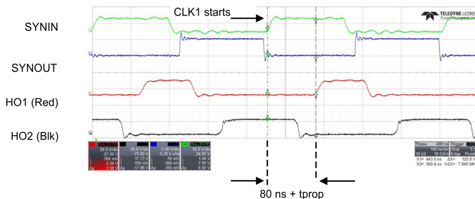
Figure 23. SYNIN and HO1 Timing (2.2 MHz)
