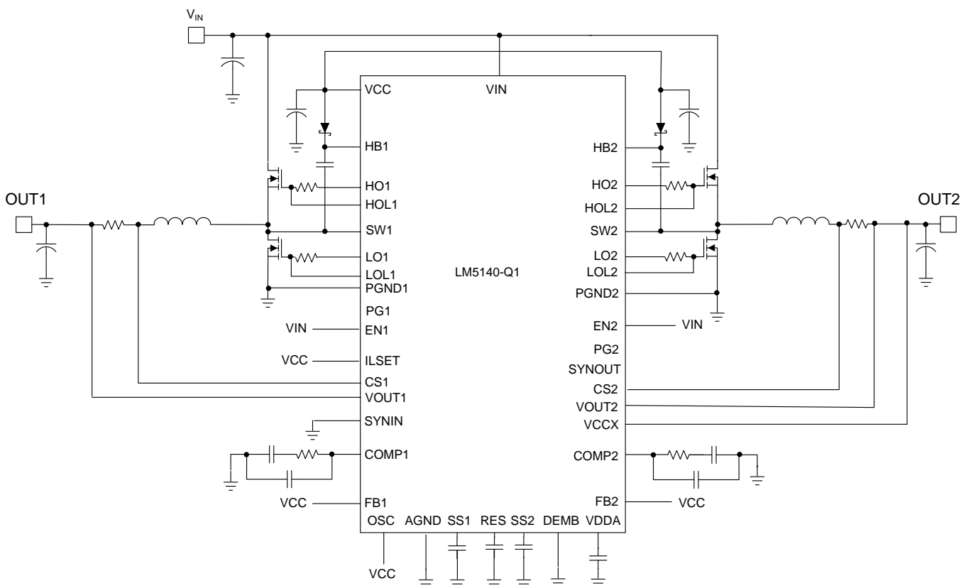
Figure 32. 12-V to 3.3-V and 5-V Converter
