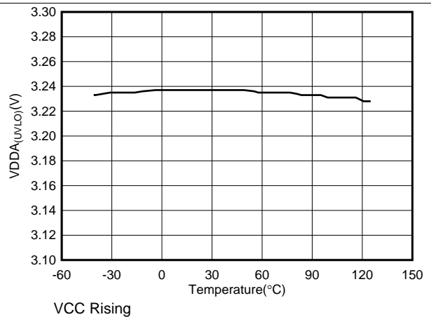
Figure 9. VDDA (UVLO) vs Temperature
