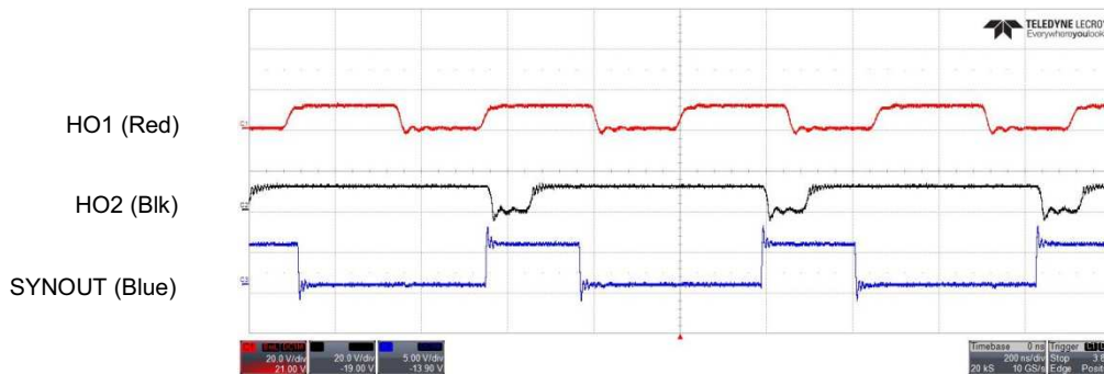
Figure 20. HO1, HO2, and SYNOUT VIN 6.41 V
