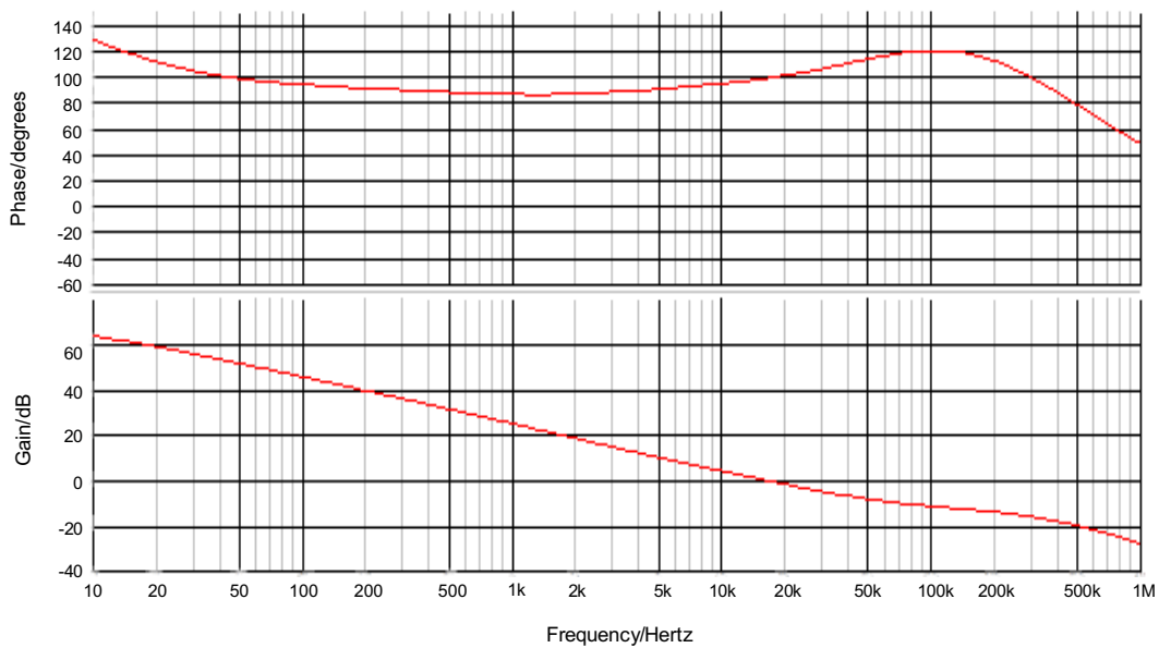
Figure 41. Open Loop Gain and Phase
