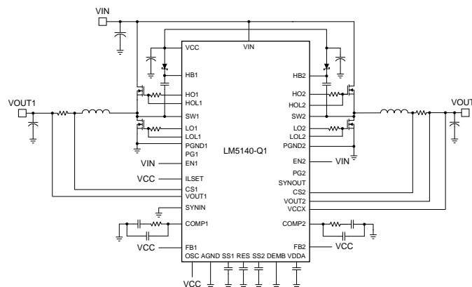
Figure 1. Simplified Schematic
