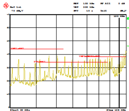
Figure 36. EMI Measurements CISPR 25 with Slew Rate Control
