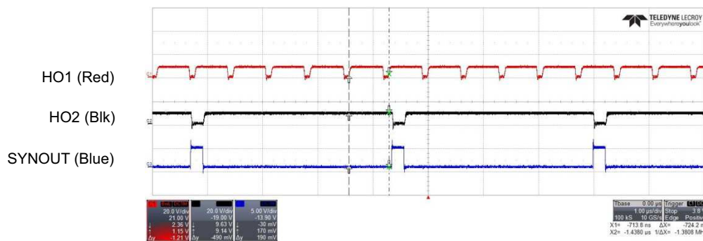
Figure 21. HO1, HO2, SYNOUT VIN 4.2 V
