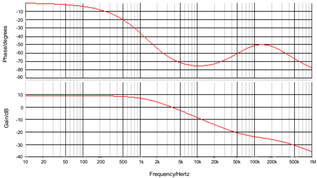
Figure 40. ( V_O/V_C ) Modulator Gain and Phase
