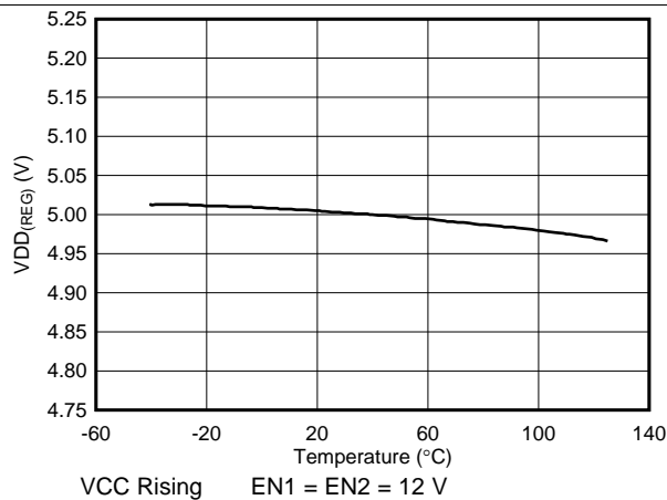
Figure 8. VDDA (REG) vs Temperature
