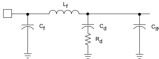
Figure 33. Input EMI Filter
