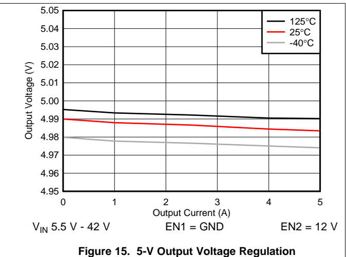
Figure 15. 5-V Output Voltage Regulation
