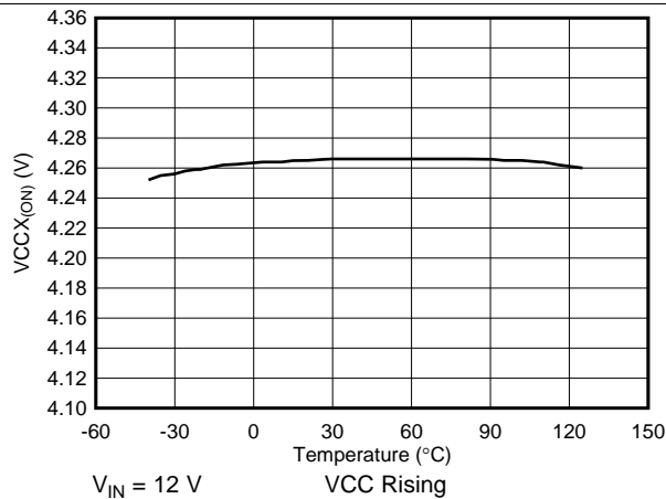
Figure 10. VCCX (ON) vs Temperature
