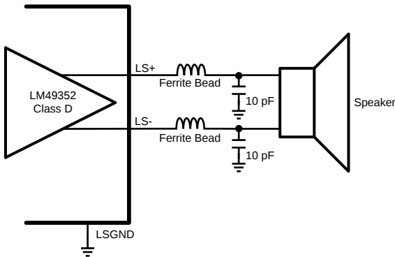
Figure 59. EMI/RFI Filter for the Class D Amplifier
