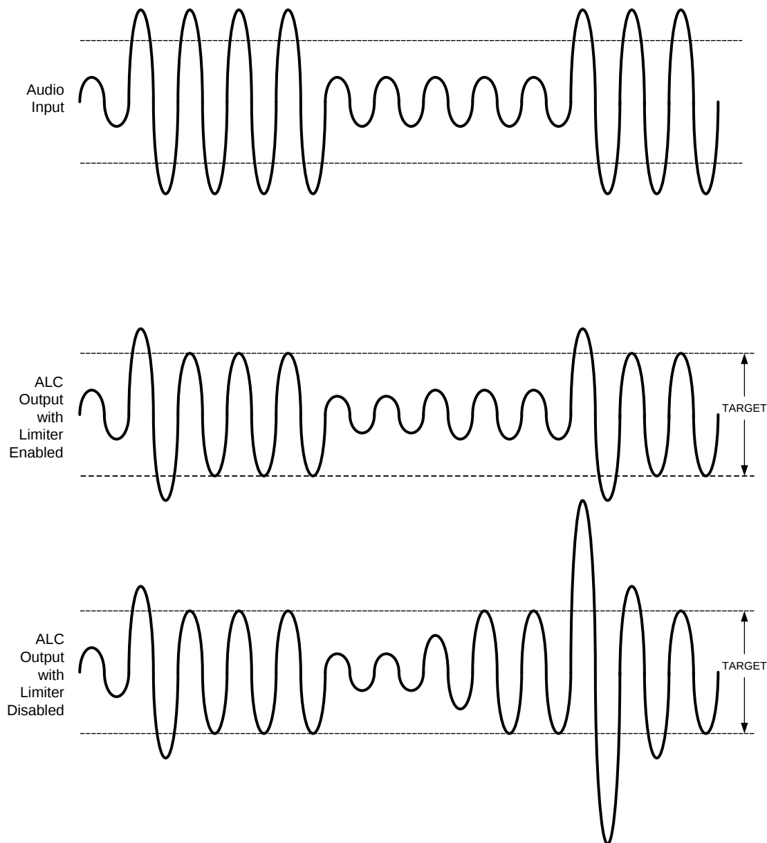
Figure 69. ALC Limiter
