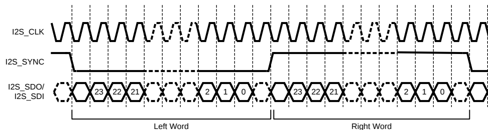
Figure 62. I²S Serial Data Format (24 bit example)
