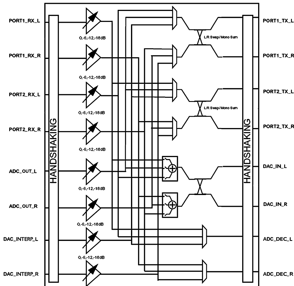
Figure 61. Digital Mixer
