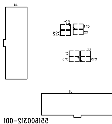
Figure 78. Bottom Silkscreen
