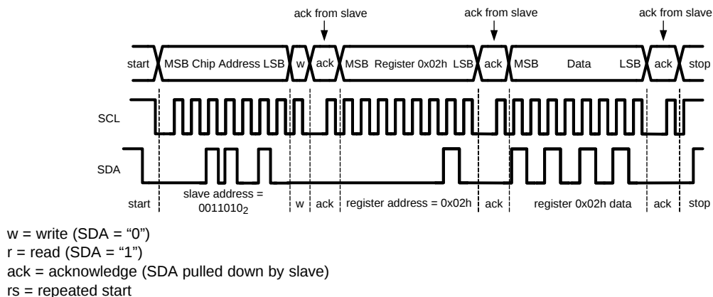
Figure 54. Example I²C Write Cycle
