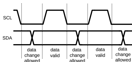
Figure 51. I 2 C Signals: Data Validity
