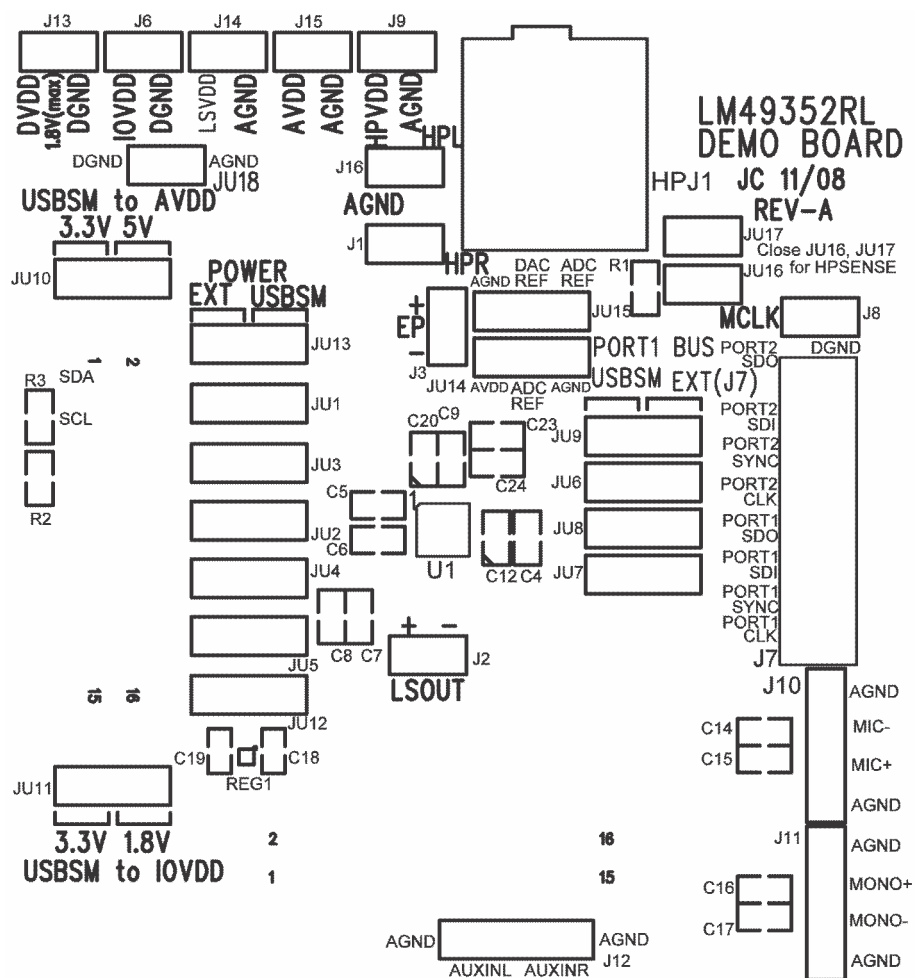
Figure 73. Top Silkscreen
