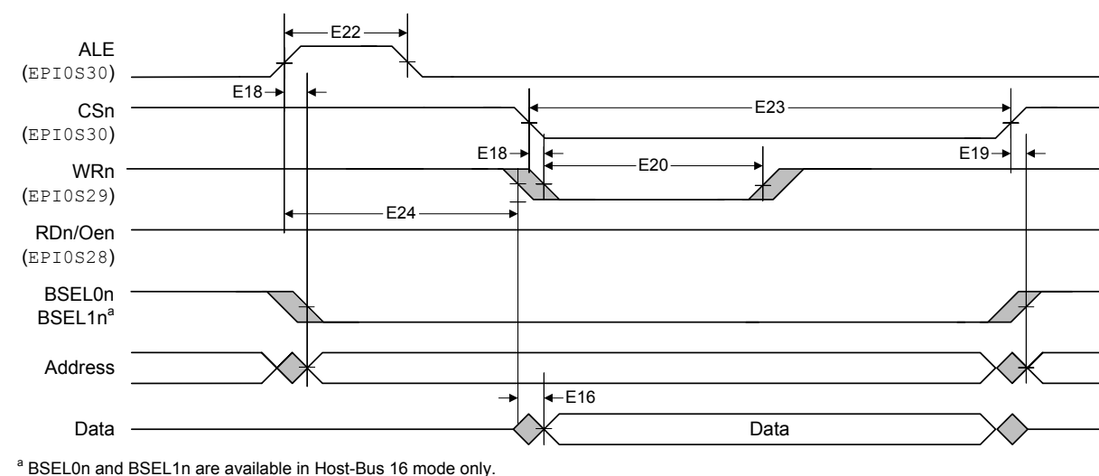
Figure 25-17. Host-Bus 8/16 Mode Write Timing
