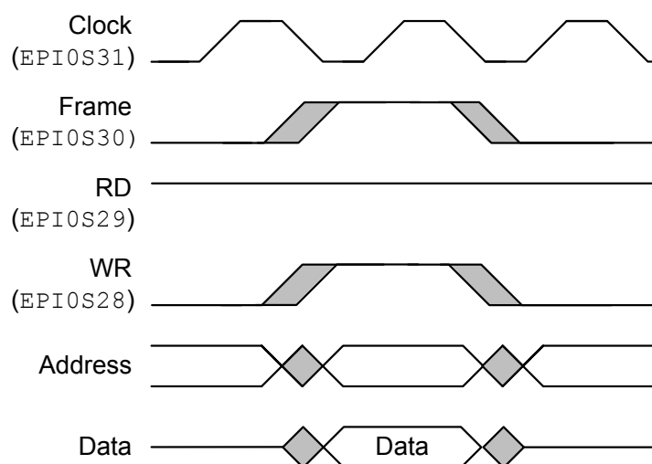
Figure 10-13. Single-Cycle Write Access, FRM50=0, FRMCNT=0, WRCYC=0
