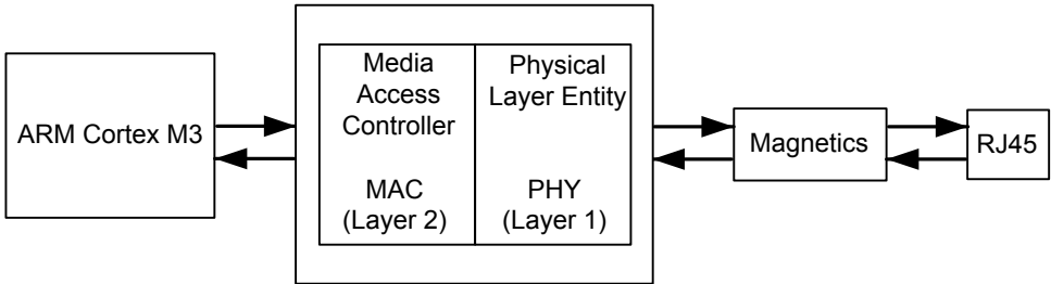
Figure 14-1. Ethernet Controller
