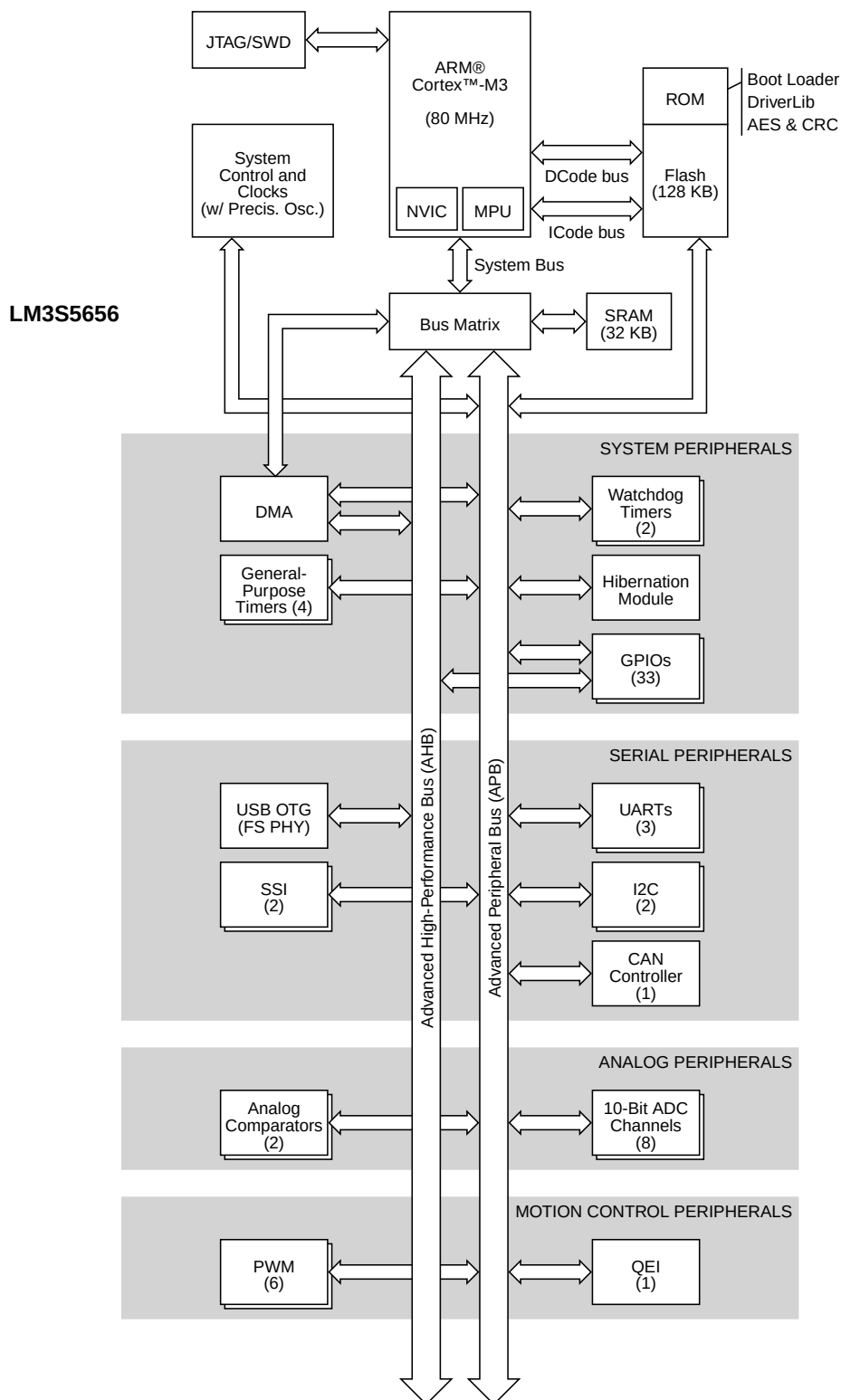
Figure 1-1. Stellaris LM3S5656 Microcontroller High-Level Block Diagram
