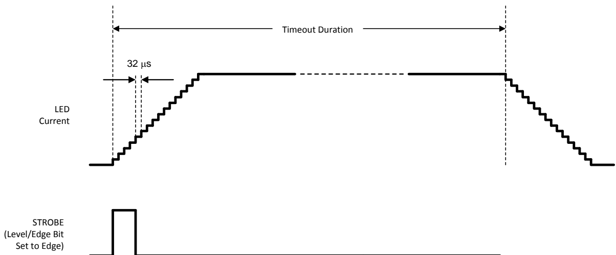
Figure 26. LED Current for STROBE (Edge Triggered, Enable Register Bit 5 = 1)
