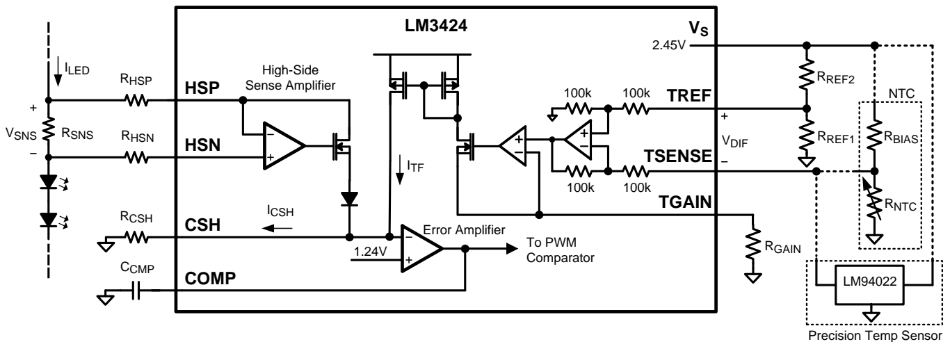
Figure 22. Thermal Foldback Circuitry
