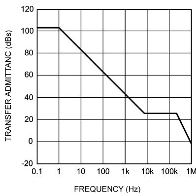
Figure 30. V_{FB} -to-Inductor Current Transfer Admittance
