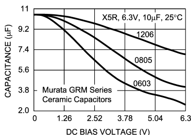
Figure 36. Capacitance vs. Applied DC Voltage
