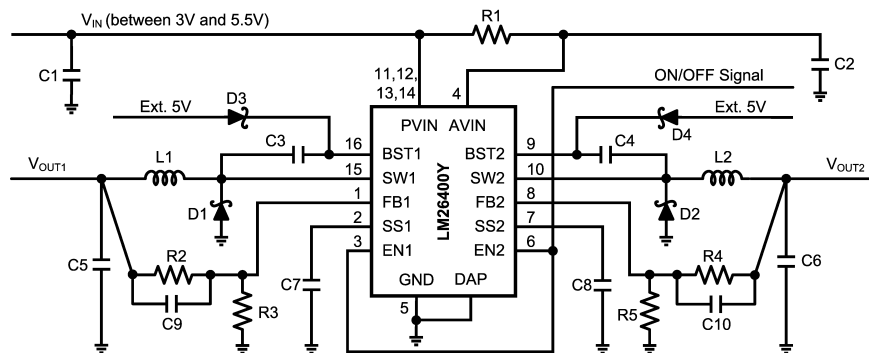
Figure 40. Example Circuit 2
