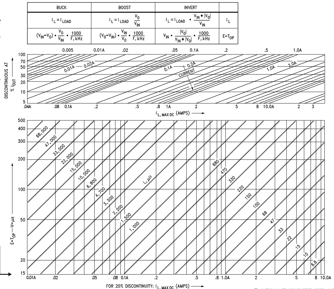
Figure 29. DC/DC Inductance Calculator
